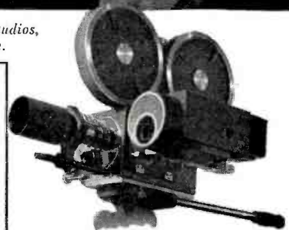
THE MAURER 16 mm . designed specifically for professional use, equipped with precision high-power focusing and view-finder. Standard equipment includes: 235° dissolving shutter, automatic fade control, view finder, sunshade and filter holder, one 400-foot gear-driven film magazine, a 60-cycle 115-volt synchronous motor, one 8-frame handcrank, power cable and a lightweight carrying case.
